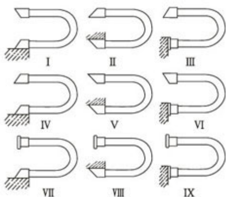
软管装配形式图 Hose assembly figure
